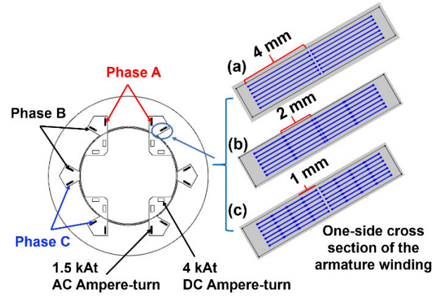
FIGURE 6. Schematic of the three different types of armature windings under investigation and the definition of the phases in the motor: (a) 4 mm-wide conductor; (b) 14/2 roebel cable; (c) striated conductor. The ampere-turns of the armature windings are 1.5 kAt (AC) while the ampere-turns of the field winding is 4 kAt (DC). The phase difference of the current for different phase in the armature winding is \frac{2}{3}\pi .
