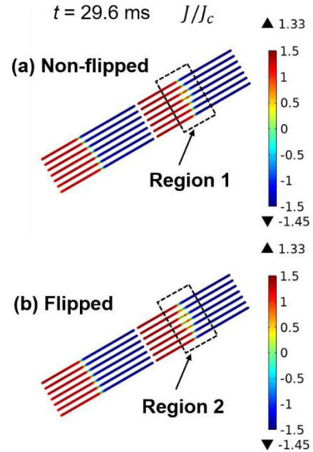
FIGURE 21. Normalized current density J/J_c distributions in C1 wound with the superpower conductor at t = 29.6 ms: (a) non-flipped and (b) flipped.
