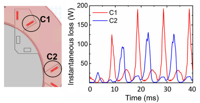
FIGURE 9. C1 and C2: two legs of one armature coil. The calculated instantaneous losses of C1 and C2 wound with 4 mm - wide (RE)BCO conductors are shown.
