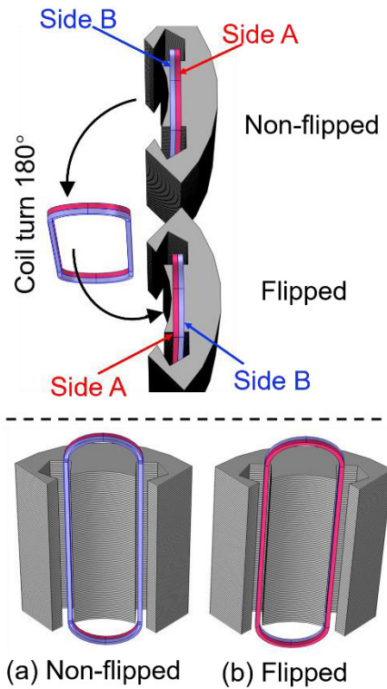
FIGURE 19. Schematic drawing of the flipping of a double racetrack armature coil: (a) non-flipped; (b) flipped.
