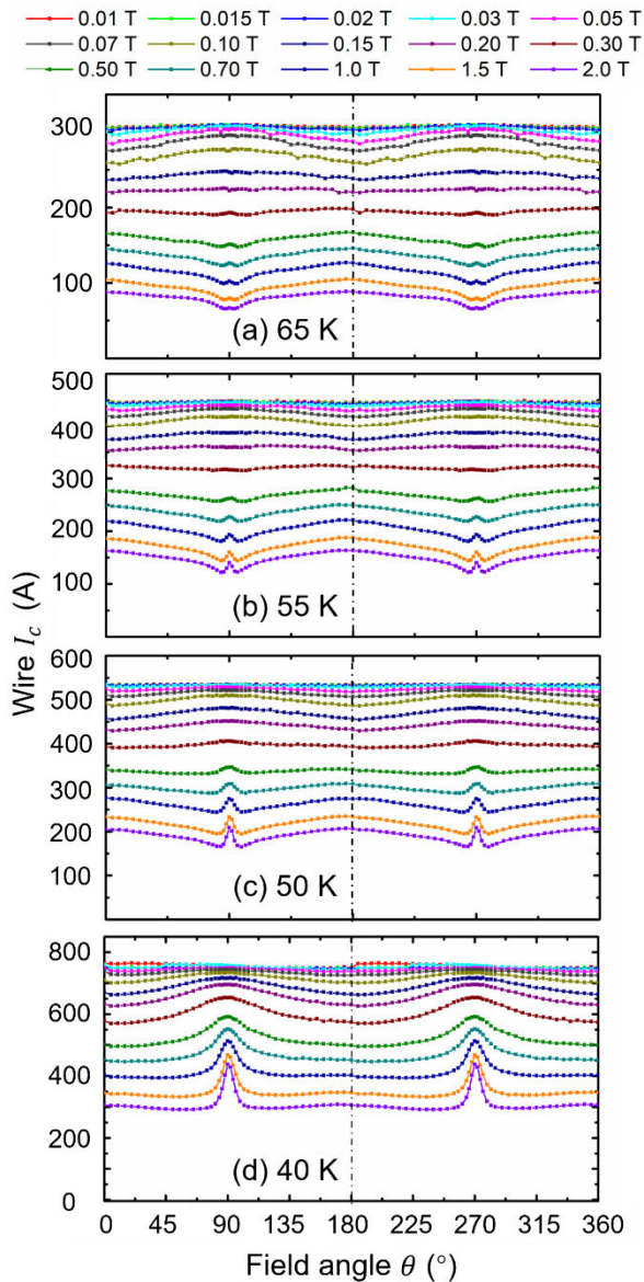
FIGURE 7. The measured I_c(B, \theta) data used in the FEM models to represent the angular magnetic field-dependence of the critical current density. Symmetry is assumed for the data from 180^\circ to 360^\circ .
