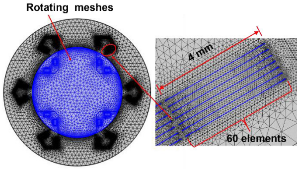
FIGURE 5. A moving mesh applied to the rotor part including rotor core, field windings and some air subdomains. A gradient mesh is applied to the edges of the (RE)BCO conductors.
