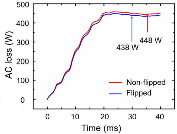
FIGURE 20. Comparison of the average AC loss between non-flipped and flipped armature windings wound assuming the asymmetric I_c(B, \theta) data of the superpower conductor.
