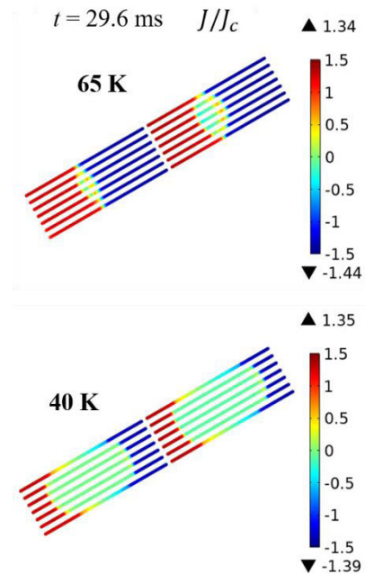
FIGURE 17. Normalized current density J/J_c distributions in C1 wound with 4 mm-wide HTS conductor at operating temperature of 65 K and 40 K.
