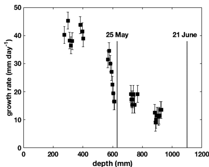
Figure 4. Banding-determined growth rates versus depth (supporting information data set S1). The vertical lines represent the assignment we have made for the neap tide on 25 May below, and the directly measured depth on 21 June. Congelation ice formation started at 150 mm.
