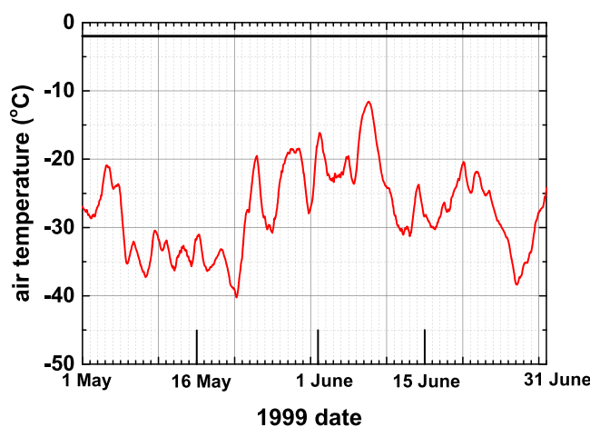
Figure 6. Air temperature versus time at Scott Base through mid-1999 [National Institute of Water and Atmospheric Research, n.d.]. The horizontal line at the top indicates a sea temperature of -1.9^{\circ}\text{C} at the base of the ice, assuming constant salinity. Note especially the sudden temperature rise occurring between 20 and 22 May, which correlates with a rapid sea-ice growth reduction near 600 mm thickness.
