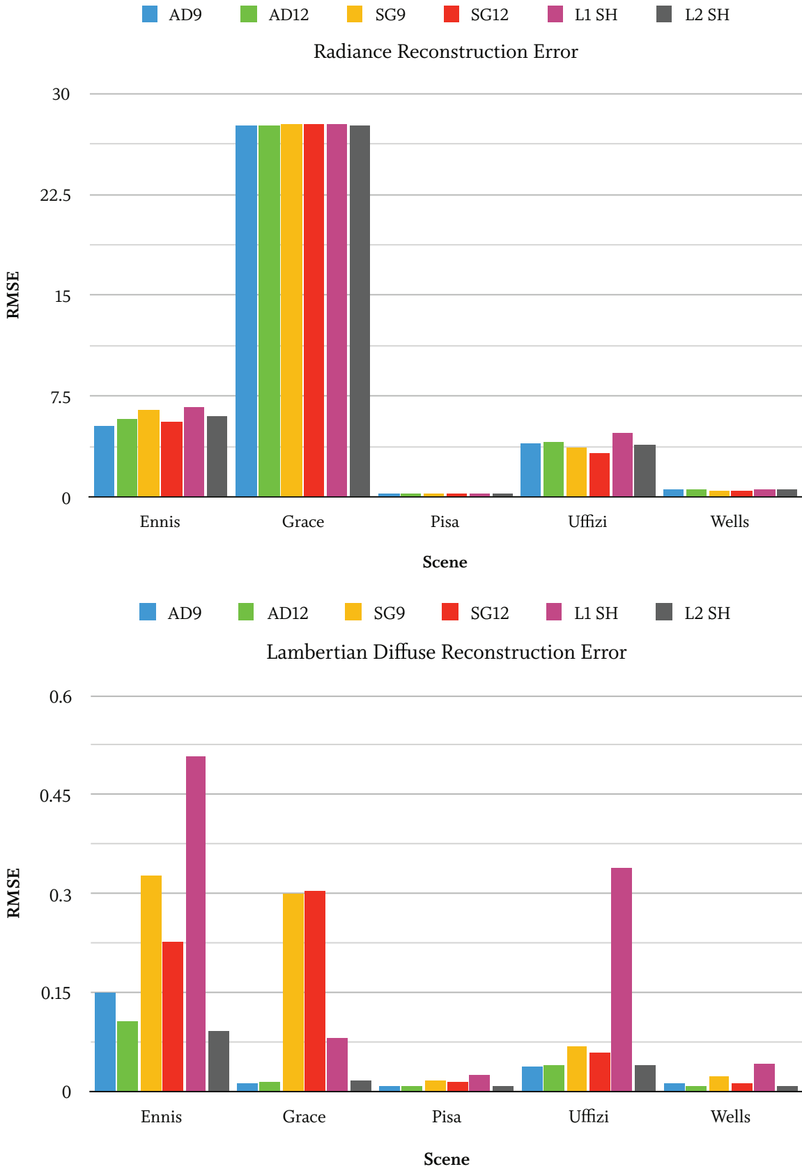
Figure C.6: Comparison graphs of reconstruction error for spherical harmonics, spherical Gaussians, and cosine-lobe Ambient Dice
