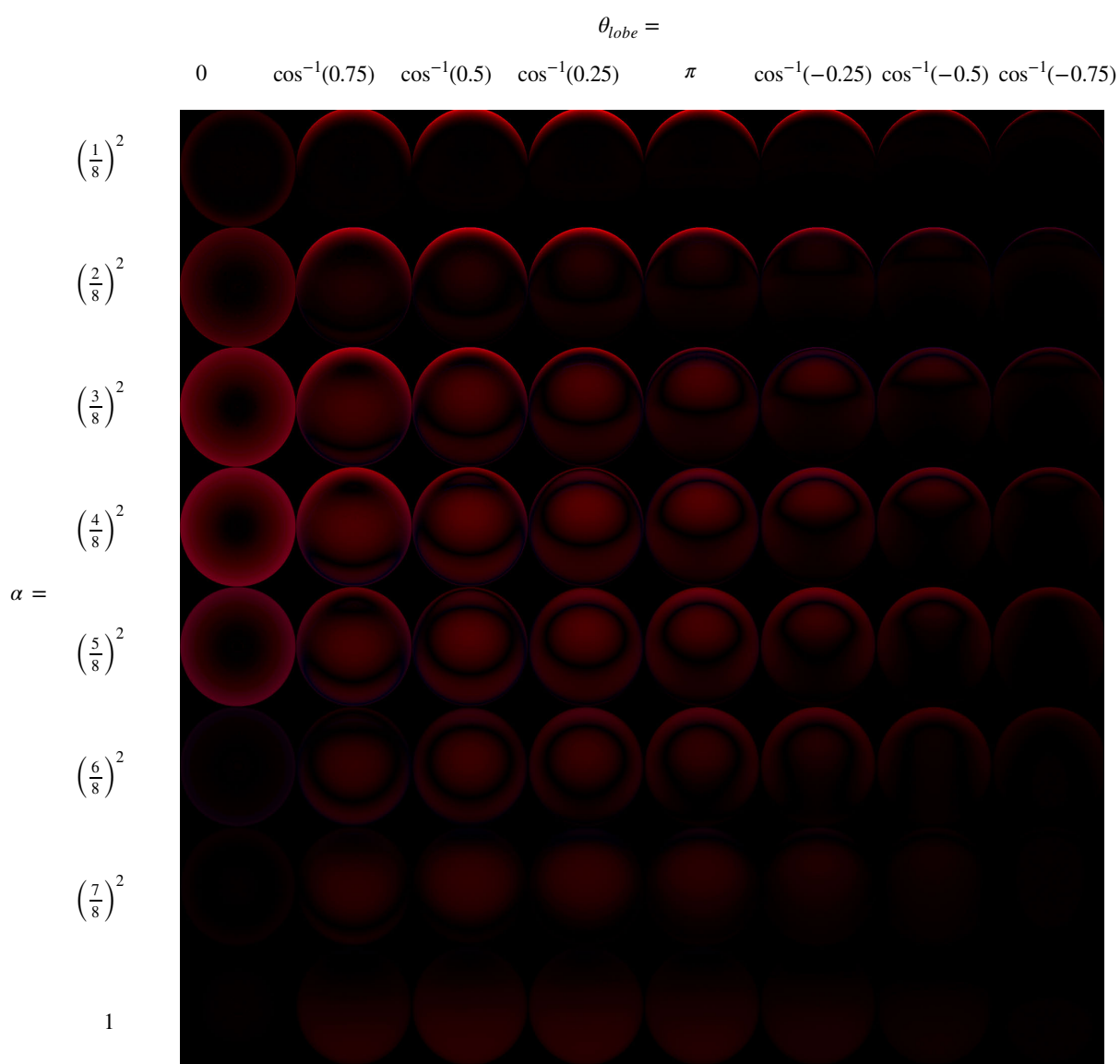
Figure 8.4: Absolute difference between the ground truth and the 2D LUT approximation for the specular response from an Ambient Dice cosine lobe with single-scattering GGX, with exposure increased by 2 EV.
