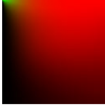
Figure 8.5: The Ambient Dice DFG texture for single-scattering GGX. N \cdot V increases to the right and \alpha increases downwards.
