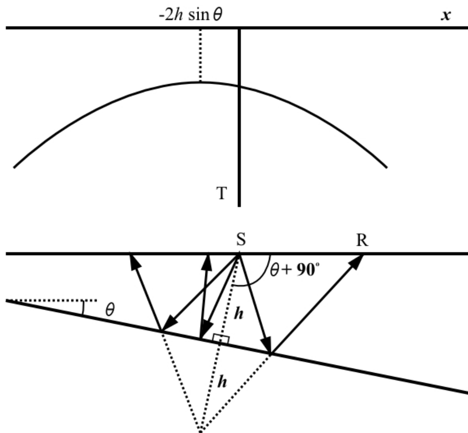
Figure B.4: Plot showing distance vs. travel time (top) for a reflection from a dipping layer. A cross-section in the earth (bottom) shows the ray paths followed.
