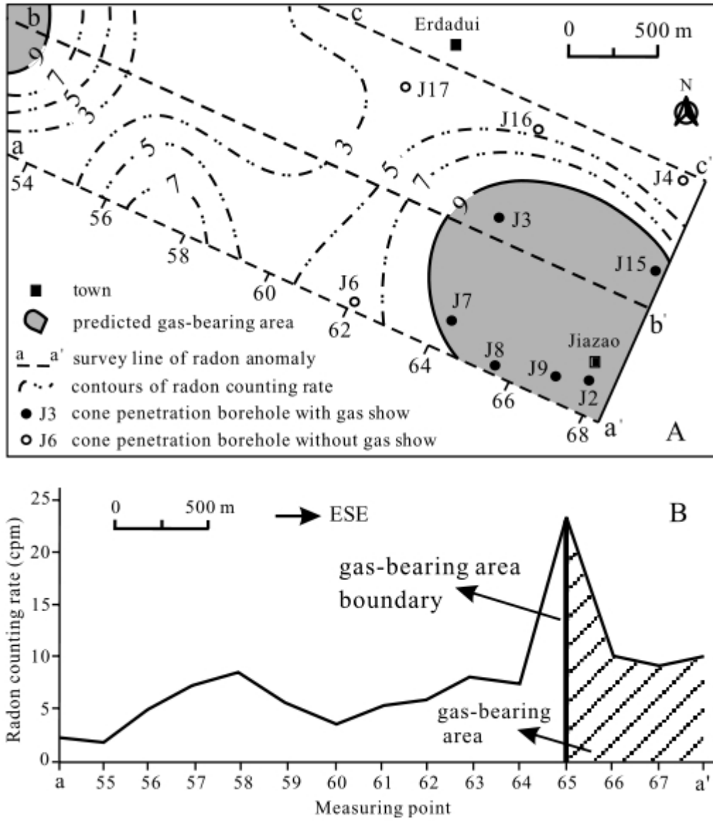
Figure 3.8: Radon anomaly in Hangzhou Bay area, eastern China. (A) Shows radon survey lines over Jiazao shallow gas field. (B) Shows radon anomaly profile (aa'). cpm = counts per minute. Reproduced from Li and Lin, [2010].
