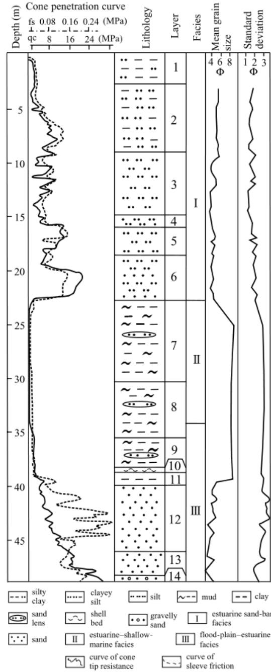
Figure 3.7: Cone penetration borehole log from the Hangzhou Bay area, eastern China. qc = cone tip resistance and fs = sleeve friction. Reproduced from Li and Lin, [2010].
