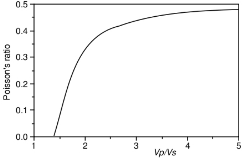
Figure 3.2: Plot showing the change in Poisson's ratio with change in V_p/V_s for an isotropic elastic medium. Reproduced from Ostrander [1984].
