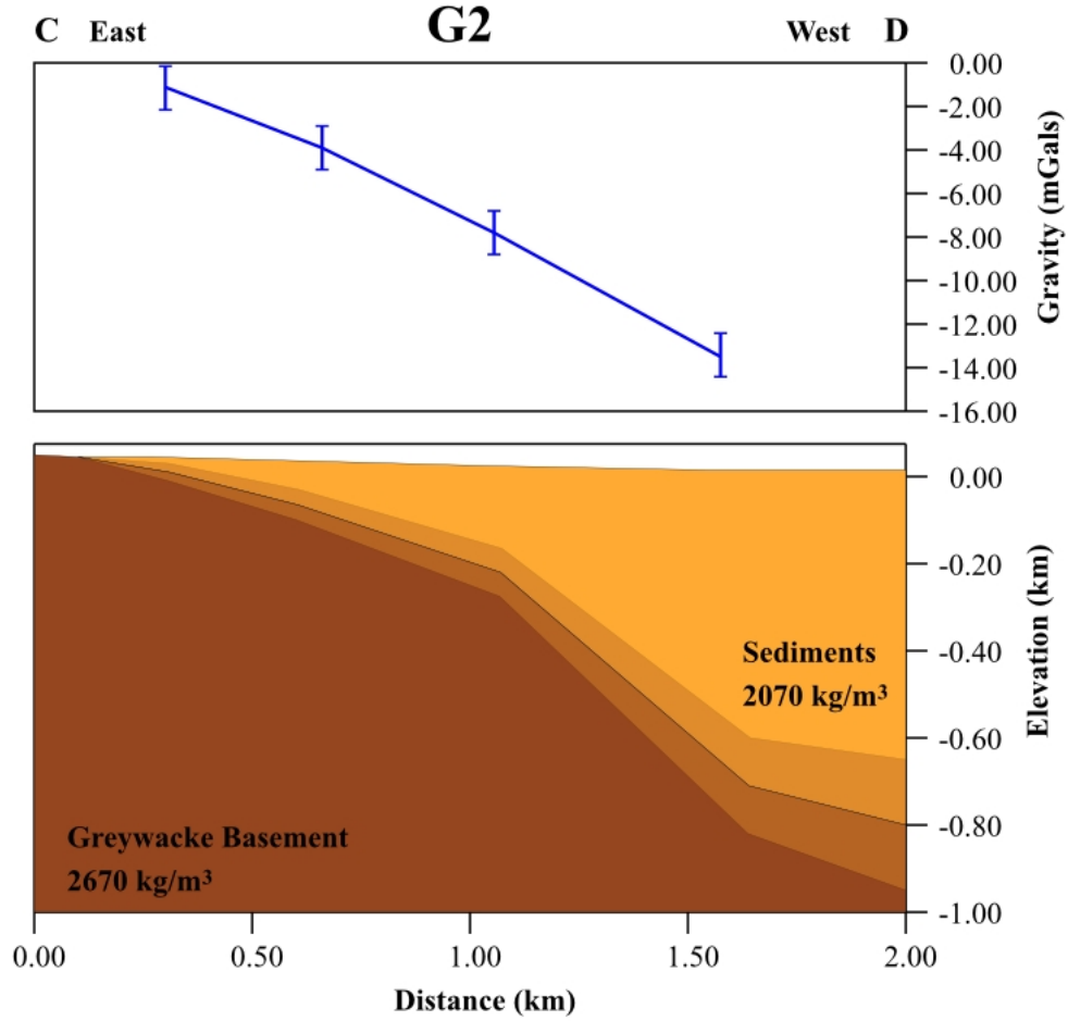
Figure 5.3: Gravity model showing basement depth along Wallace Road. The location of the gravity profile is shown in figure 5.1. Observed gravity with uncertainties (blue error bars) and modelled gravity (blue line) are shown. Densities of \rho = 2070 \text{ kg/m}^3 for sediments and \rho = 2670 \text{ kg/m}^3 for greywacke basement rock were used. Greywacke basement is found to dip gently west then drop sharply near the west end of the line, as in the parallel survey along Muhunua East Road (figure 4.3). Greywacke basement reaches the surface at the eastern end of the profile where it meets the edge of the Tararua range front, resulting in a residual gravity field of -0.5 mGal. Apart from where it is faulted between 1.1–1.6 km on the profile, the steepest basement dip observed is 14 \pm 4^\circ west.
