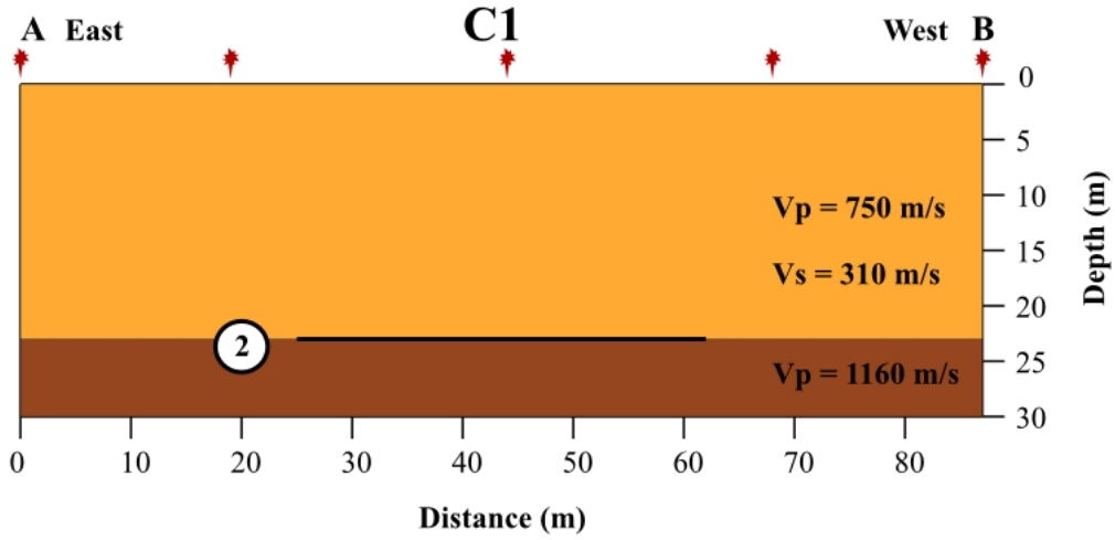
Figure 6.4: Diagram showing layer depths and velocities for survey C1. Refraction/reflection 2 from the layer boundary at 23 m depth is shown. The heavy black line shows the extent of the interface that was imaged.
