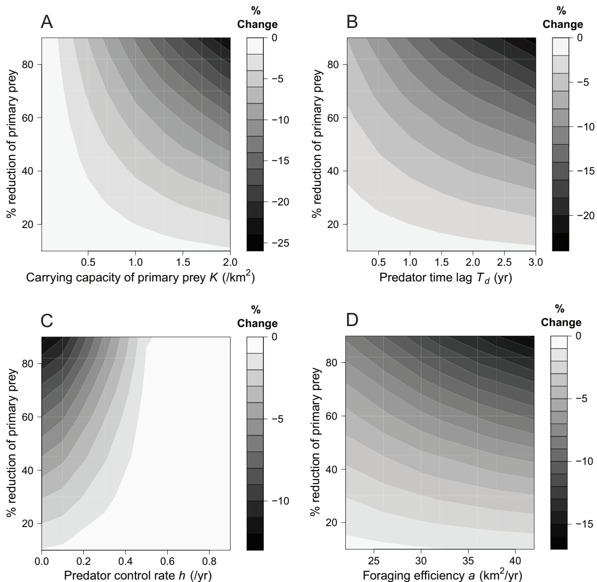
Figure 3: Change in abundance of the secondary prey (as a percentage of its equilibrium value P_2^* : 100 \times (P_2^{\min} - P_2^*)/P_2^* ) as a function of the primary prey's reduction (%) and the carrying capacity of the primary prey (A), the time lag of the predator's numerical response (B), the rate of predator control (C), and the foraging efficiency of the predator (D). Results are mean values of 1,000 iterations of stochastic parameter sampling from equations (1)–(3) (corresponding standard deviations are presented in fig. A1, available online), except point values are used for values from the X- and Y-axes.
