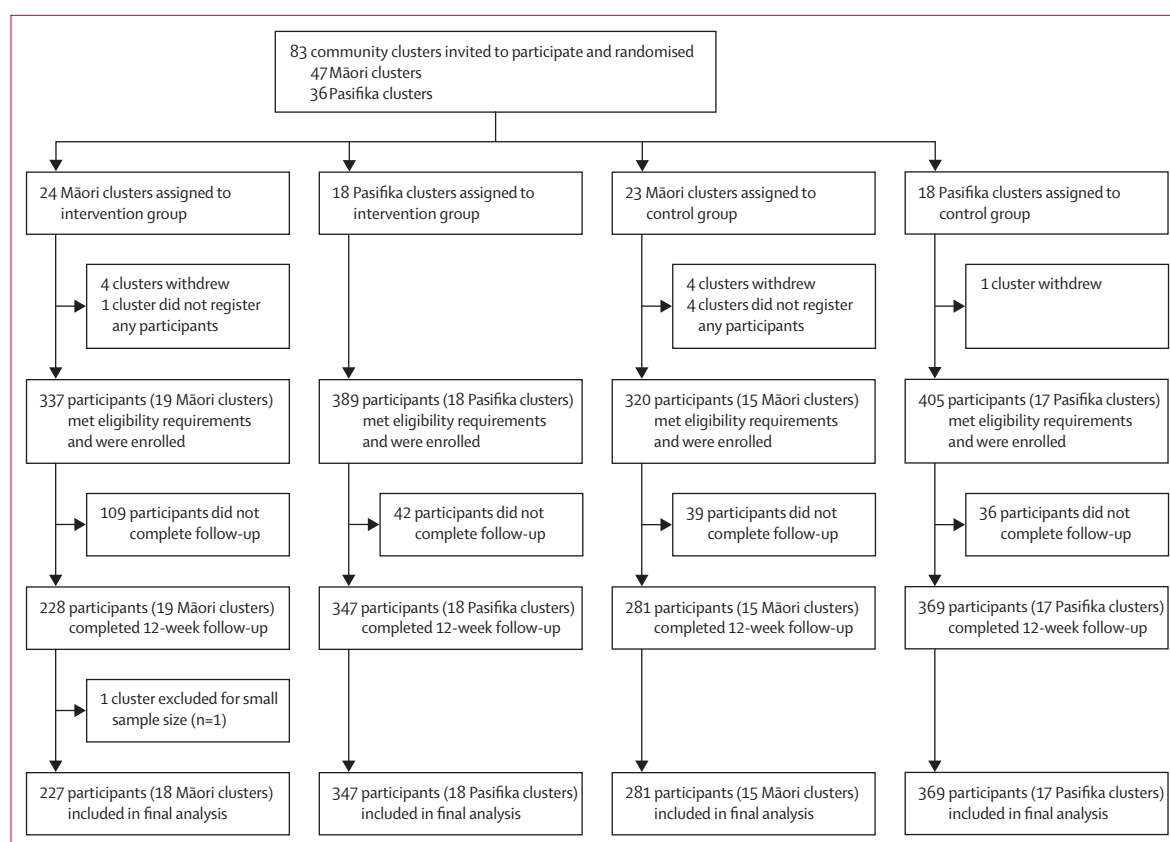
Figure 2: Trial profile
